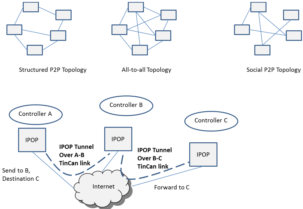
Figure 3.6: IPOP enables different controllers to implement different overlay topology maintenance and routing for different usage scenarios. Each controller binds to an IPv6 VNIC with a unique address in the overlay, allowing identifier-based routing through multiple intermediaries. Neighboring controllers can communicate using transports layered upon IPv6, thereby facilitating the programming of controller-controller protocols.
